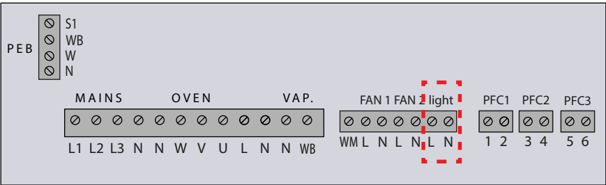
Connection for light 230 V AC
