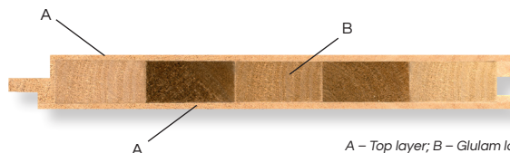
A – Top layer; B – Glulam layer
