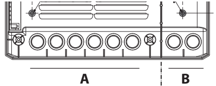
A. Mains cable, cables for heating, light etc. B. Low-voltage lines, e.g. sensor, S-Bus lines.
