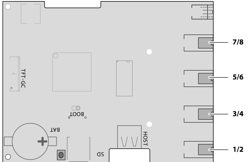
EmoTouch 3 circuit board – jacks
