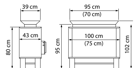
Optional frame for extra 30 - 45 kg sauna stones. Optional cover protection rail with direct mounting on the heater.
